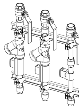
ISIMET Rack Assembly
