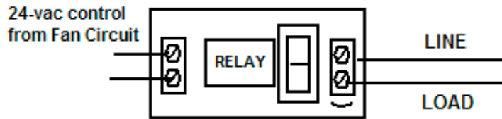
Typical 120-vac Wiring where fan is single speed
